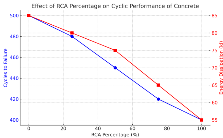
Figure 3. Relationship Between RCA Proportion and Cyclic Resistance of Concrete
